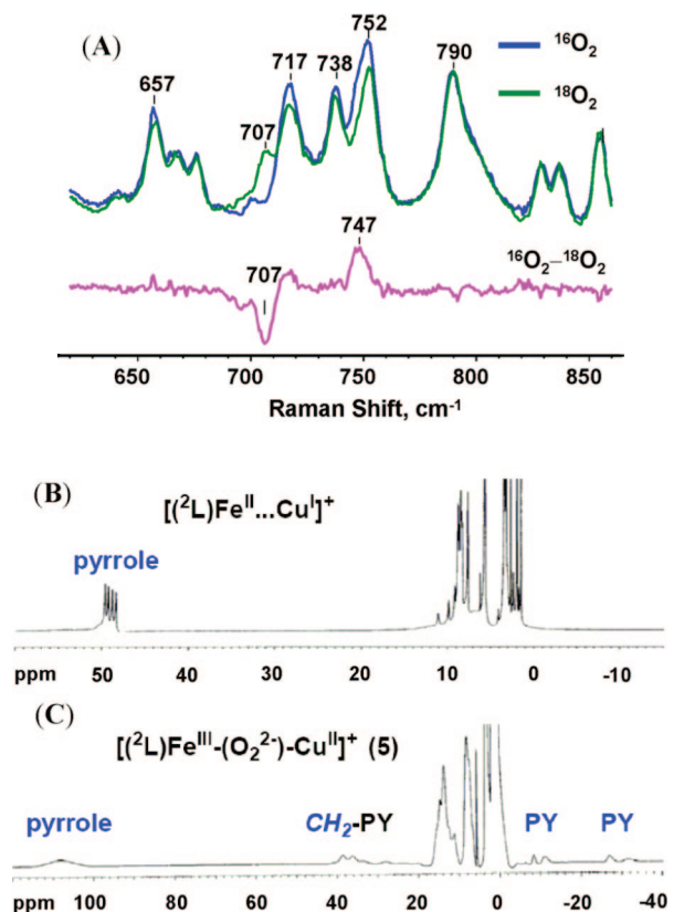
FIGURE 2. (A) Resonance Raman spectra of [(^{2}\text{L})\text{Fe}^{\text{III}}-(\text{O}_2^{2-})-\text{Cu}^{\text{II}}]^+ (5), formed by the oxygenation of [(^{2}\text{L})\text{Fe}^{\text{III}}\dots\text{Cu}^{\text{I}}]^+ with ^{16}\text{O}_2 and ^{18}\text{O}_2 , respectively. The lower part represents the difference spectrum showing \nu_{\text{O-O}} = 747 \text{ cm}^{-1} and \Delta(^{18}\text{O}_2) = -40 \text{ cm}^{-1} . ^1\text{H} NMR spectra (acetone- d_6 ) of (B) [(^{2}\text{L})\text{Fe}^{\text{III}}\dots\text{Cu}^{\text{I}}]^+ ( \delta_{\text{pyrrole}} \sim 50 \text{ ppm} ; room temperature) and (C) [(^{2}\text{L})\text{Fe}^{\text{III}}-(\text{O}_2^{2-})-\text{Cu}^{\text{II}}]^+ (5) ( \delta_{\text{pyrrole}} \sim 110 \text{ ppm} ; -90 \text{ }^\circ\text{C} ).
